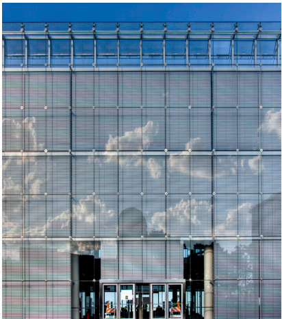
Figure 3 (left): The VS-1 glazing system is used along the east facade which uses cast stainless steel fittings to clamp the IGUs.
