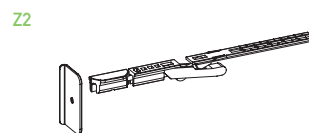
DOUBLE PLUNGER KIT cod. CEACCSTD00003 p. 136
